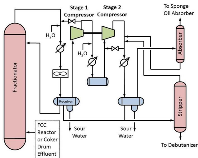
Figure 10: Wet Gas Separators
