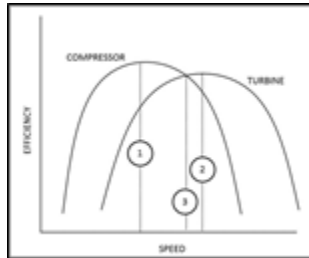
Figure 17: Compressor and Turbine Speed vs Efficiency Curves
