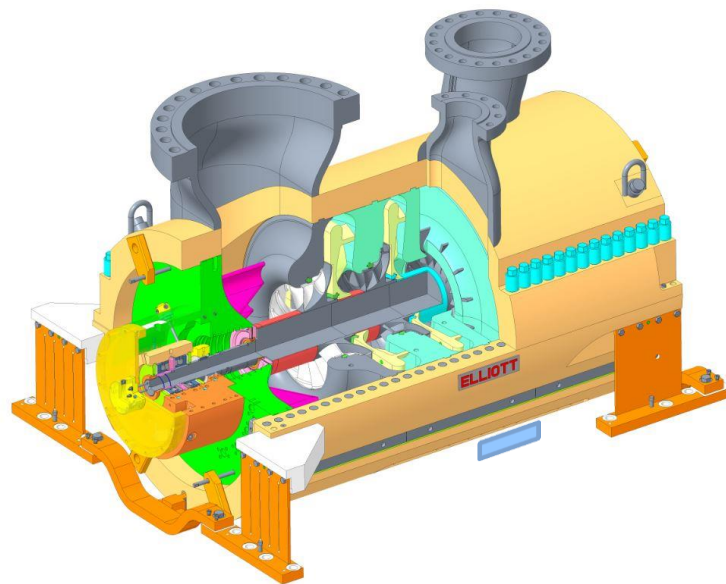
Figure 14: Alkylation Refrigeration Compressor
