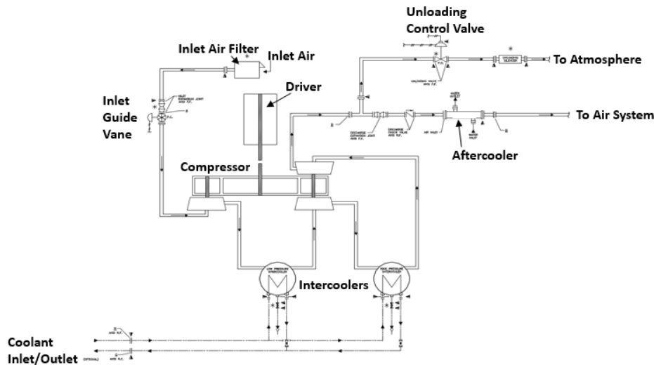
Figure 15: Integrally Geared Compressor Layout
