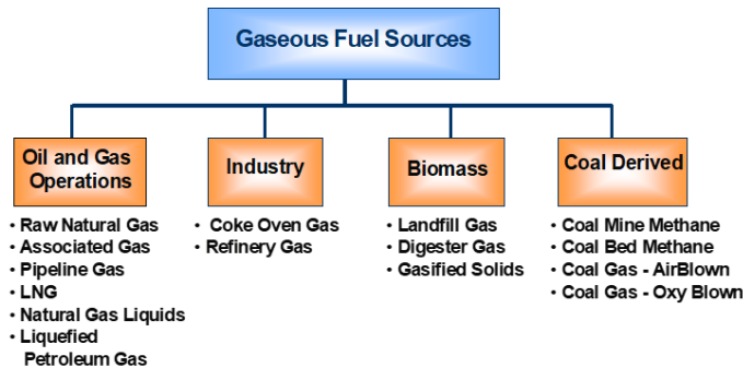
Figure 23: Gas Turbine Fuel Sources
