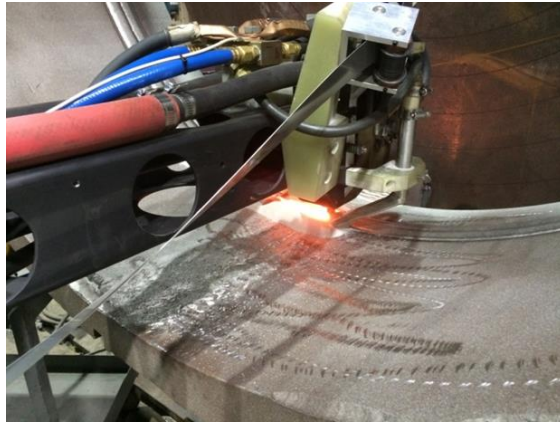
Figure 26: Electro Slag Welding (ESW) of Strip on Carbon Steel Compressor Flange Face
